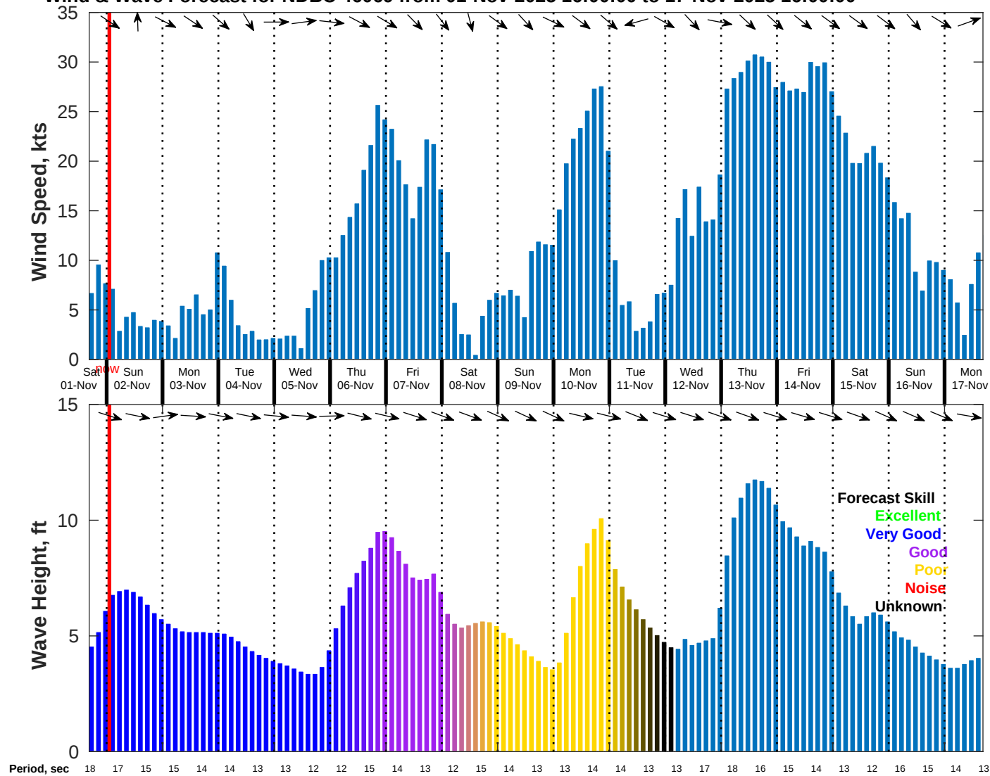
Wind & Wave Forecast for NDBC 46069 from 01-Nov-2025 16:00:00 to 17-Nov-2025 16:00:00
