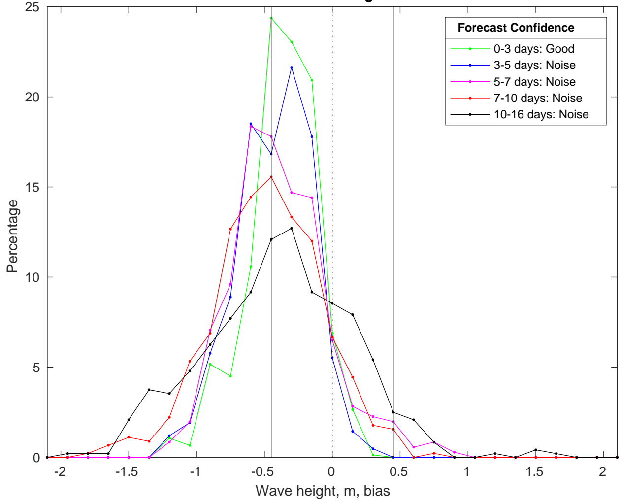
NDBC 46215 vs GFS Waves Bias Histogram: 02-Nov-2025
