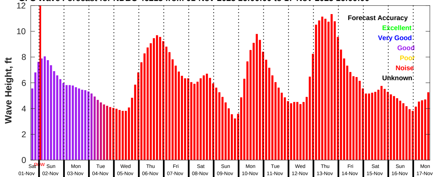
GFS Wave Forecast for NDBC 46215 from 01-Nov-2025 16:00:00 to 17-Nov-2025 16:00:00
