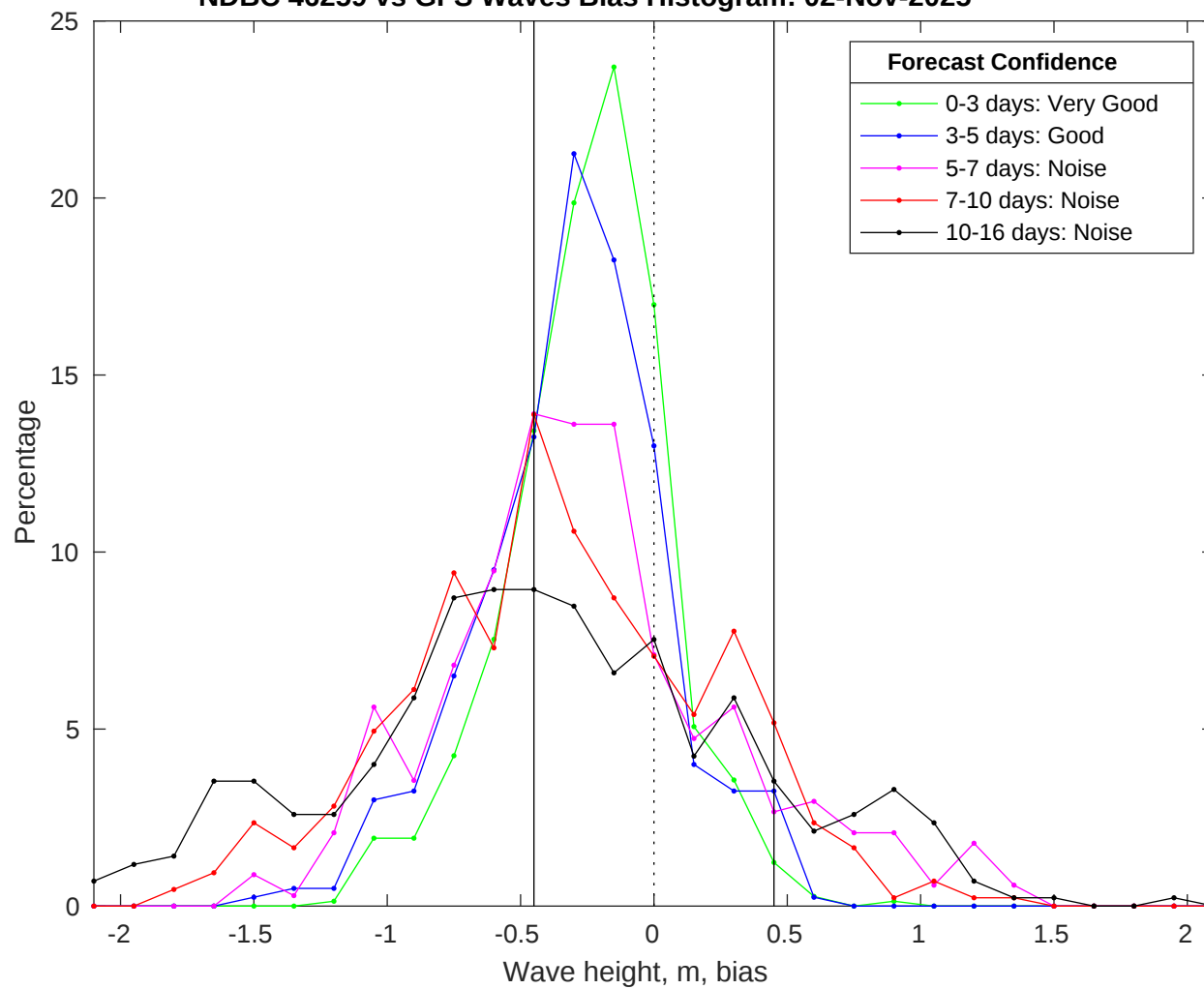
NDBC 46259 vs GFS Waves Bias Histogram: 02-Nov-2025
