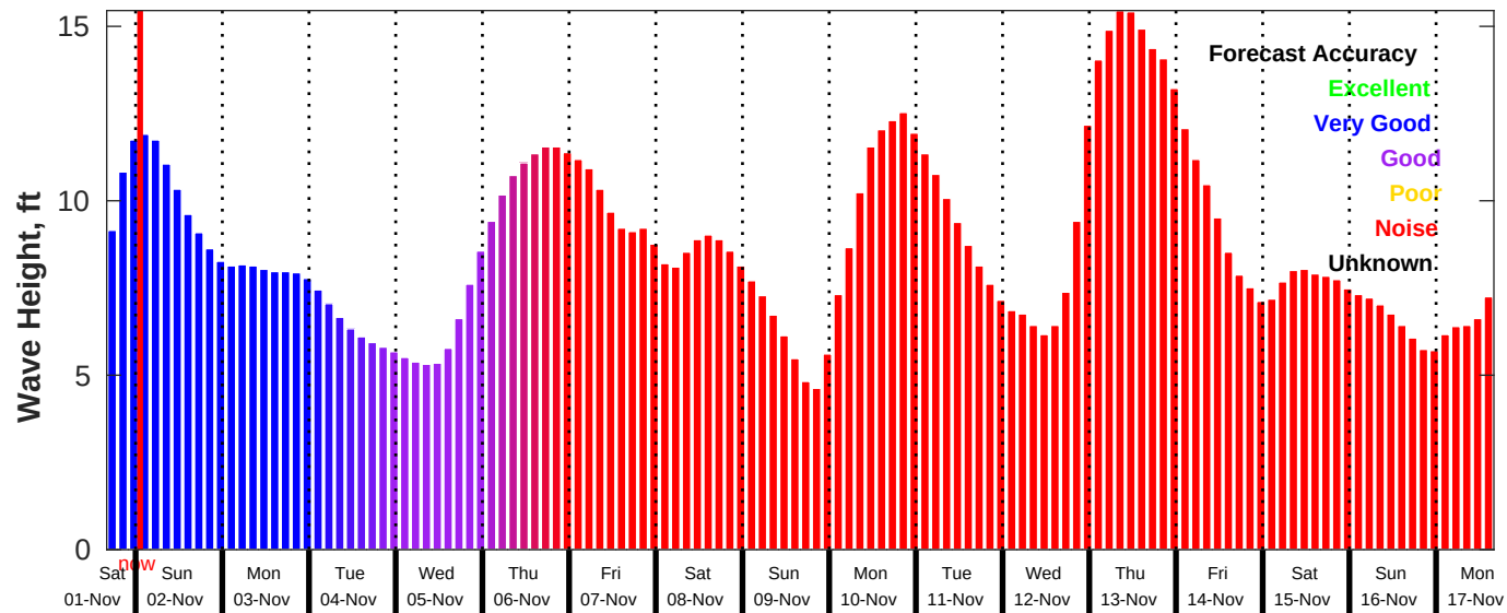
GFS Wave Forecast for NDBC 46259 from 01-Nov-2025 16:00:00 to 17-Nov-2025 16:00:00
