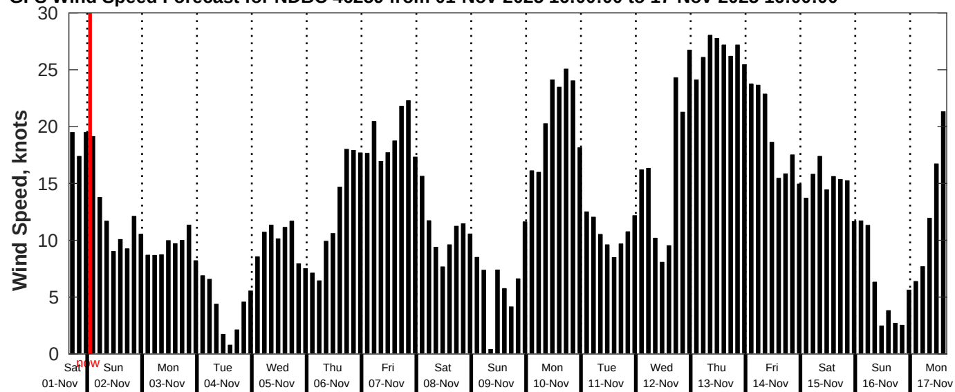
GFS Wind Speed Forecast for NDBC 46259 from 01-Nov-2025 16:00:00 to 17-Nov-2025 16:00:00
