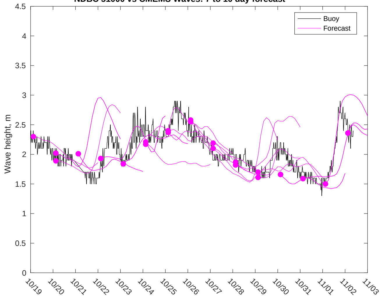
NDBC 51000 vs CMEMS Waves: 7 to 10 day forecast
