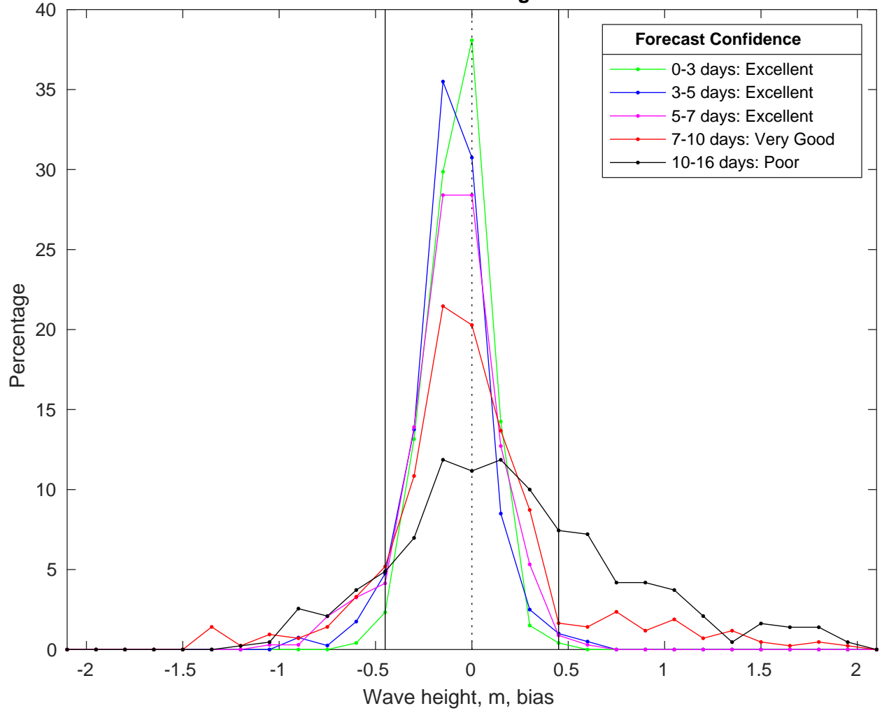
NDBC 51000 vs GFS Waves Bias Histogram: 02-Nov-2025
