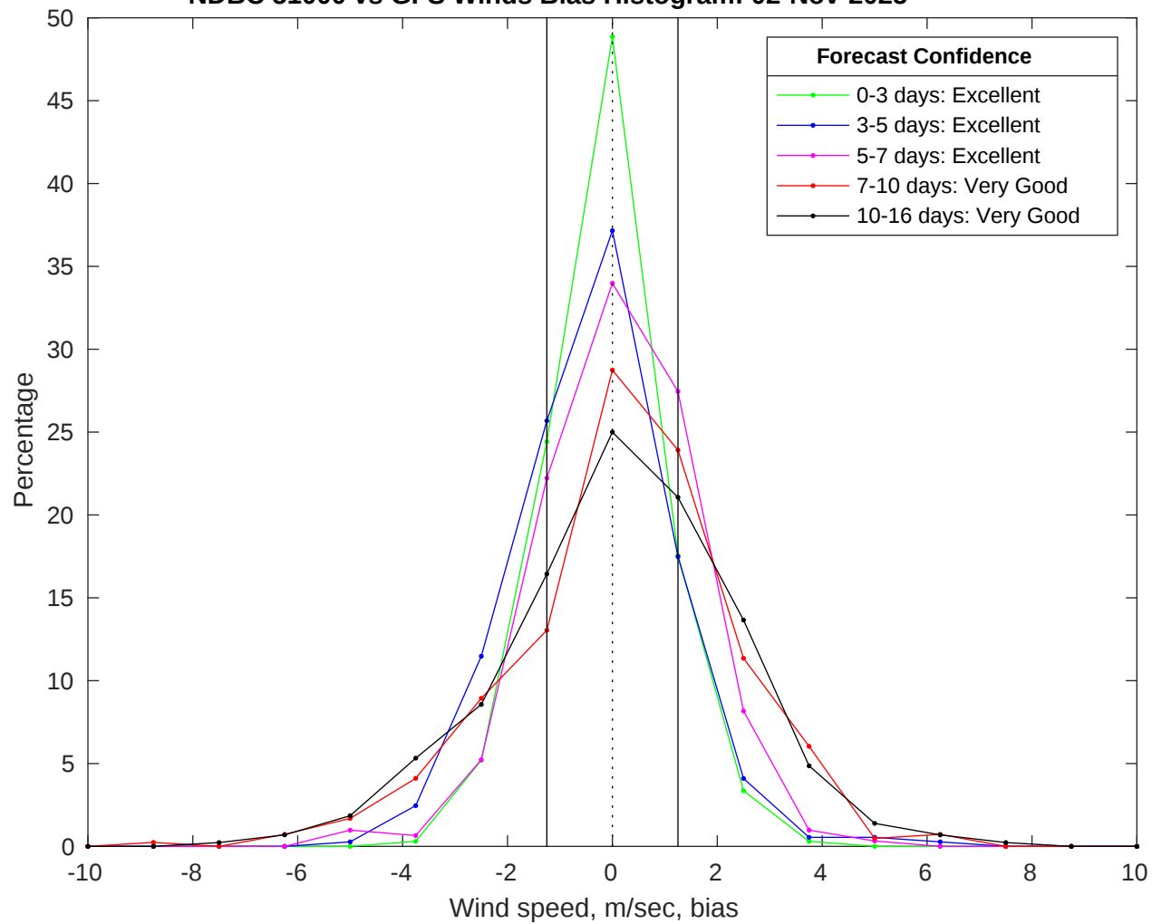
NDBC 51000 vs GFS Winds Bias Histogram: 02-Nov-2025
