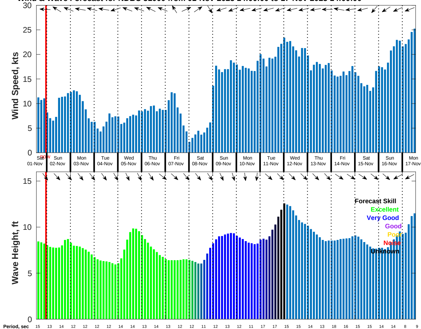
Wind & Wave Forecast for NDBC 51000 from 01-Nov-2025 14:00:00 to 17-Nov-2025 14:00:00
