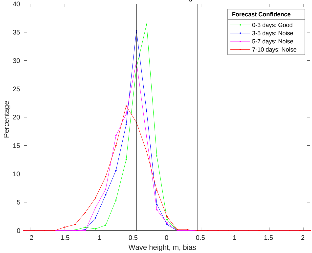
NDBC 51209 vs CMEMS Waves Bias Histogram: 02-Nov-2025
