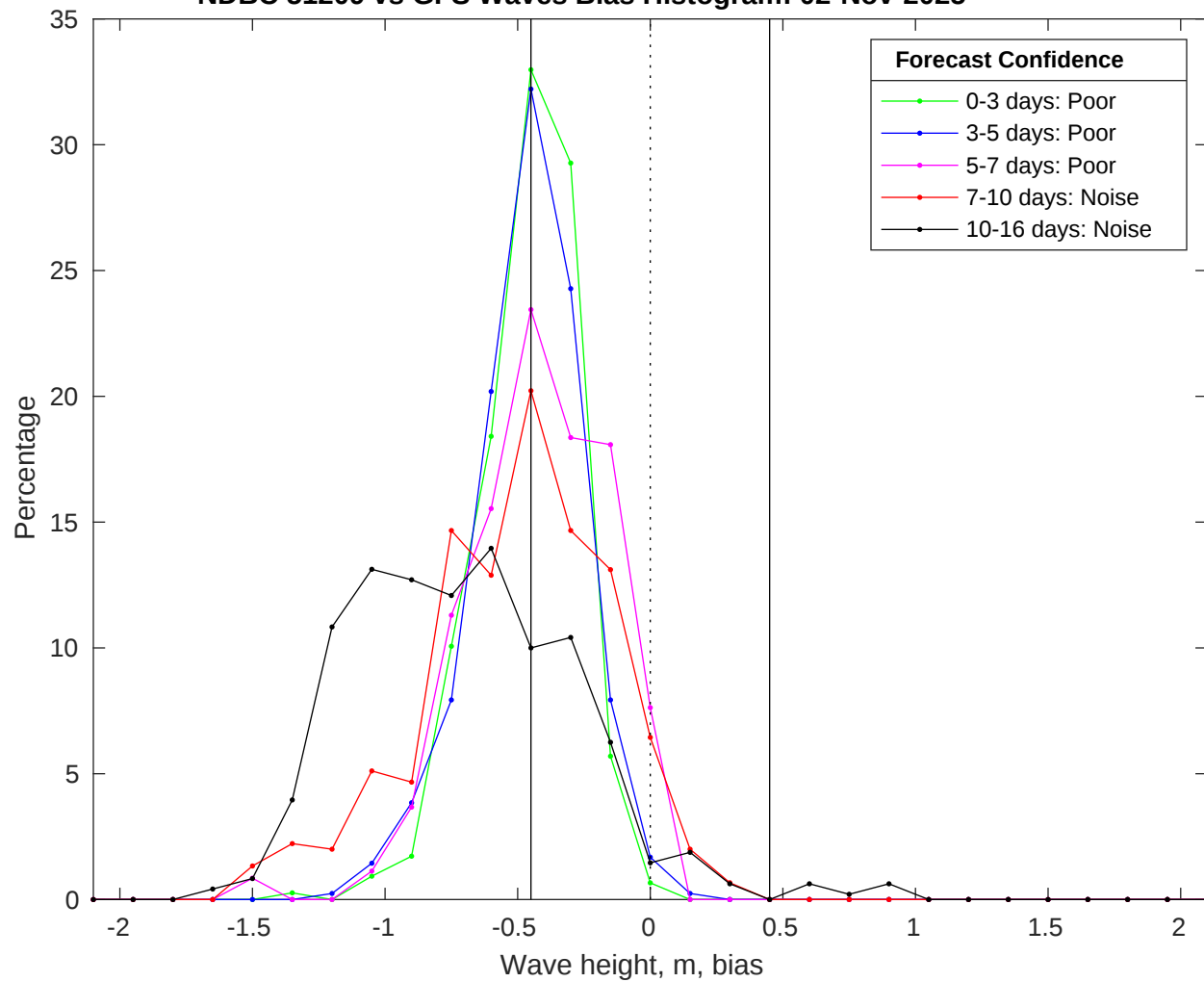
NDBC 51209 vs GFS Waves Bias Histogram: 02-Nov-2025
