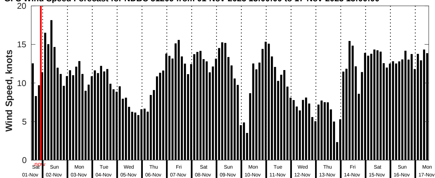
GFS Wind Speed Forecast for NDBC 51209 from 01-Nov-2025 13:00:00 to 17-Nov-2025 13:00:00
