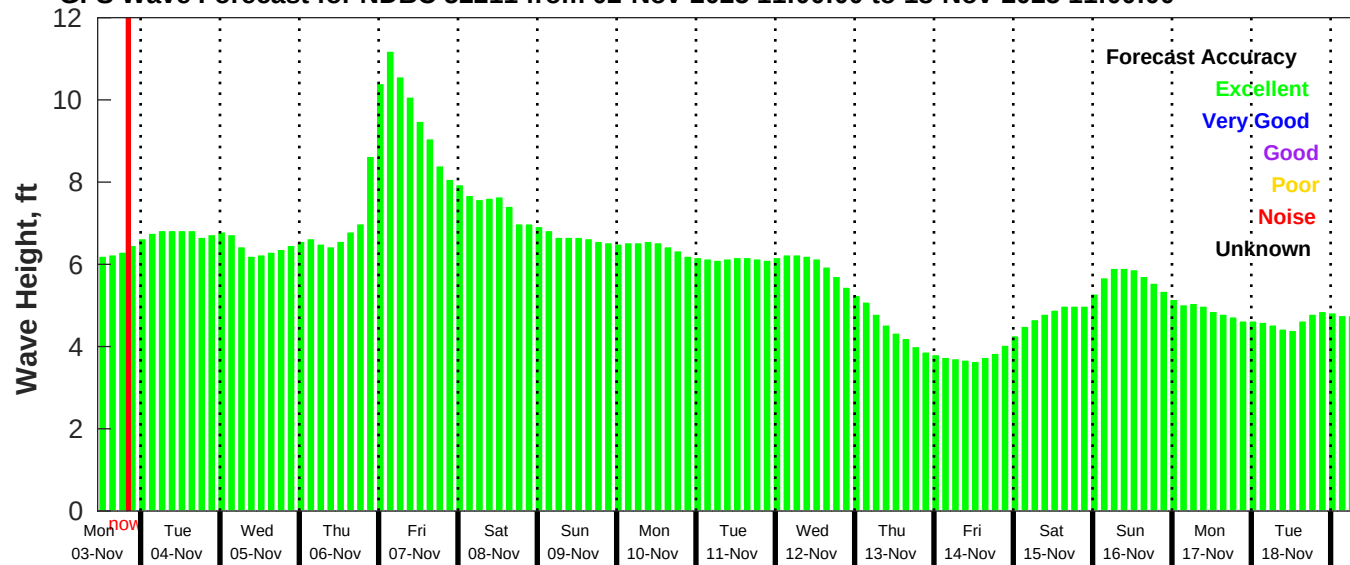
GFS Wave Forecast for NDBC 52211 from 02-Nov-2025 11:00:00 to 18-Nov-2025 11:00:00
