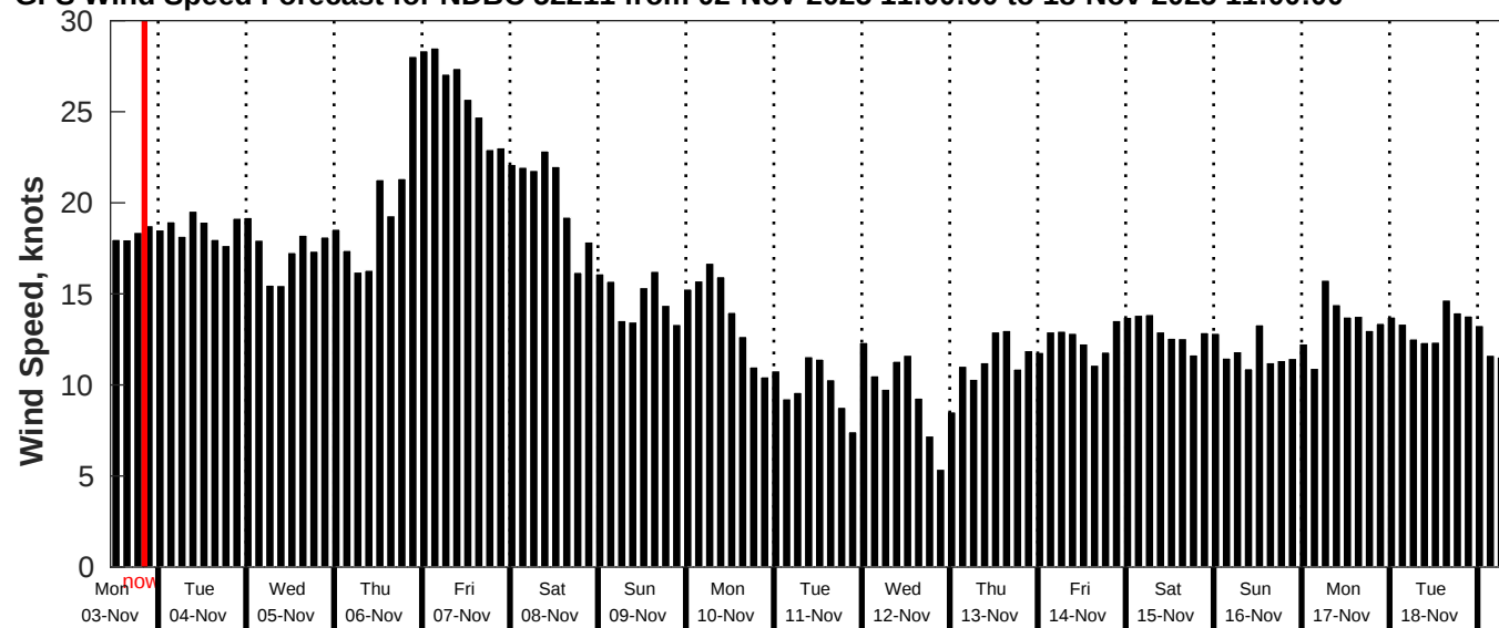
GFS Wind Speed Forecast for NDBC 52211 from 02-Nov-2025 11:00:00 to 18-Nov-2025 11:00:00
