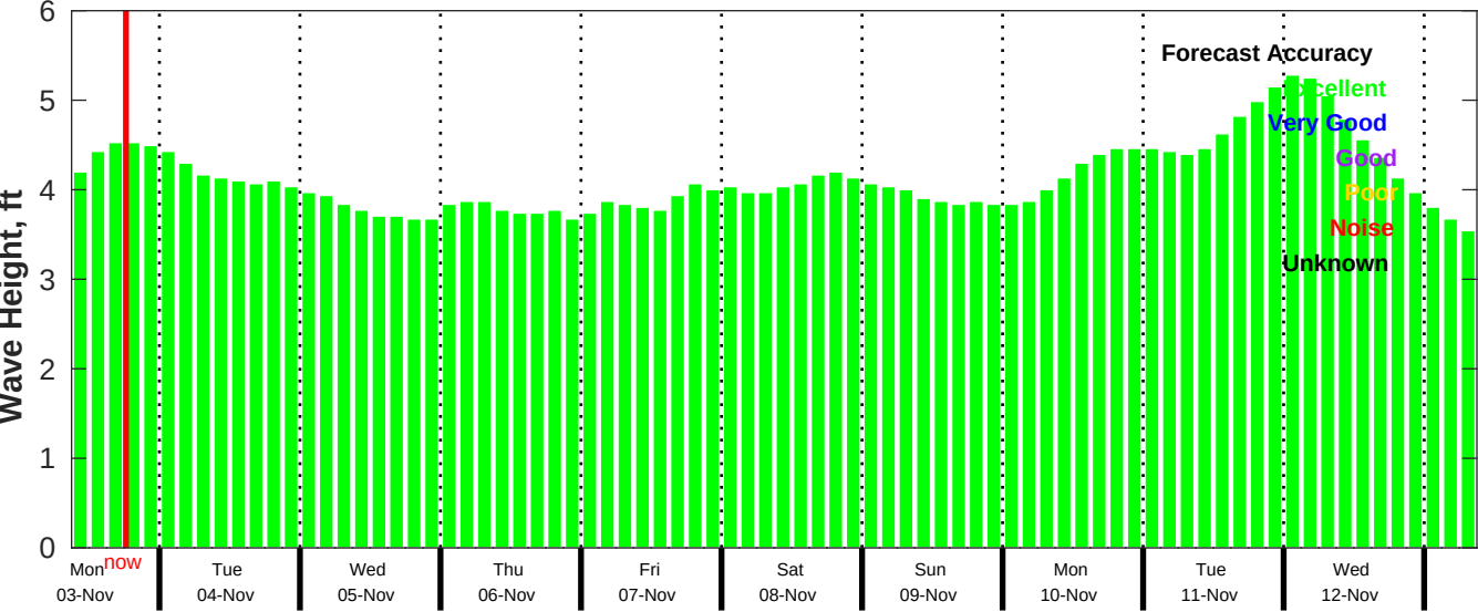
CMEMS Wave Forecast for NDBC 52212 from 02-Nov-2025 09:00:00 to 12-Nov-2025 09:00:00
