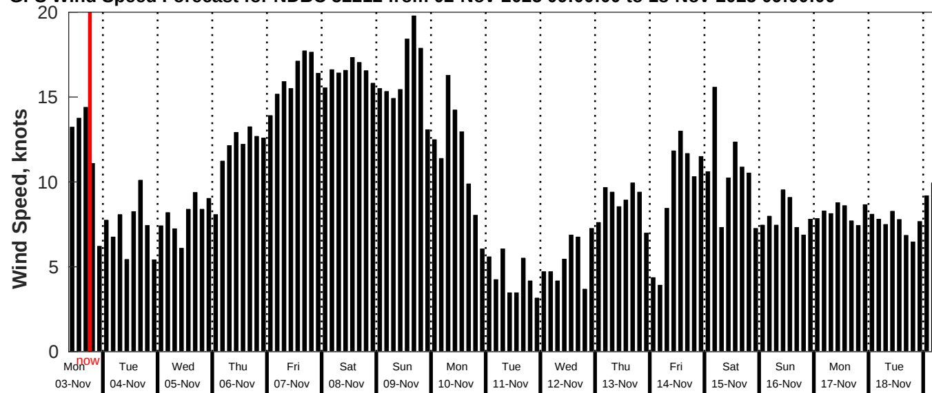
GFS Wind Speed Forecast for NDBC 52212 from 02-Nov-2025 09:00:00 to 18-Nov-2025 09:00:00
