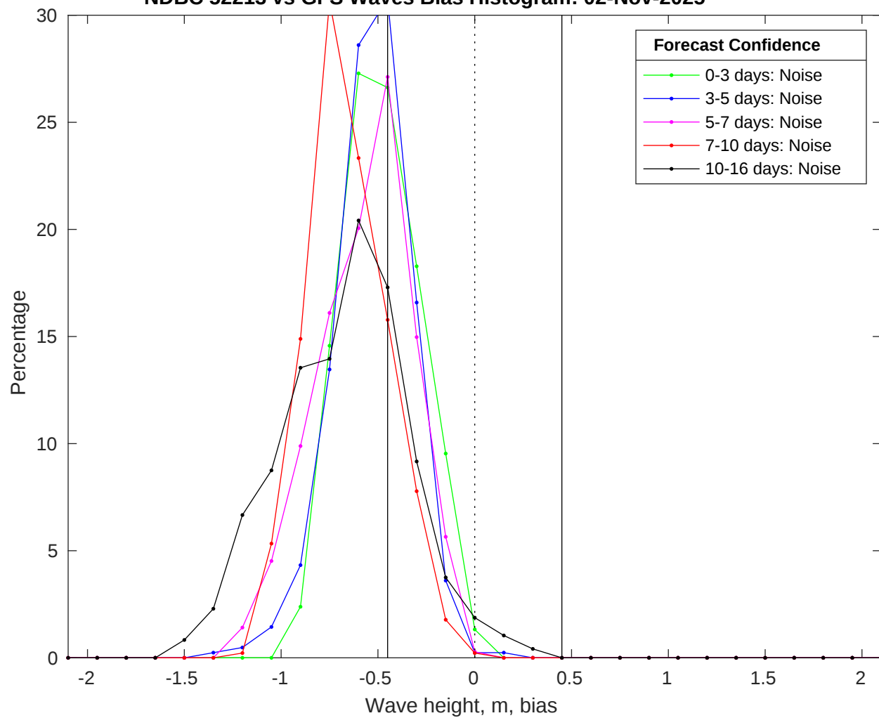
NDBC 52213 vs GFS Waves Bias Histogram: 02-Nov-2025
