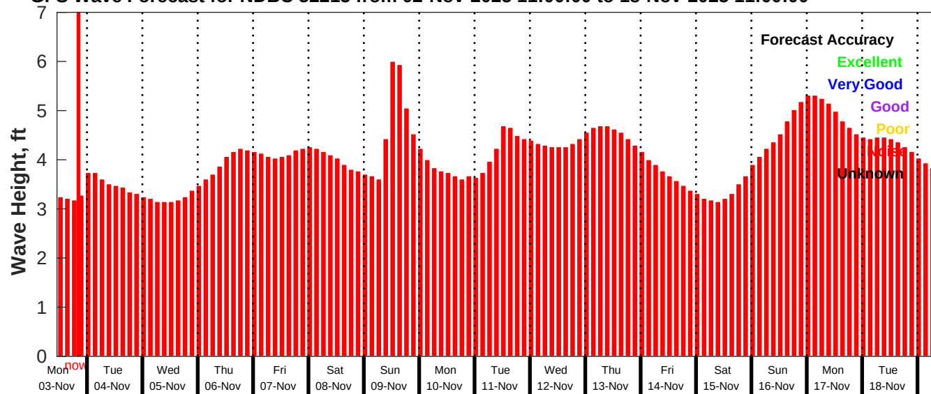
GFS Wave Forecast for NDBC 52213 from 02-Nov-2025 11:00:00 to 18-Nov-2025 11:00:00
