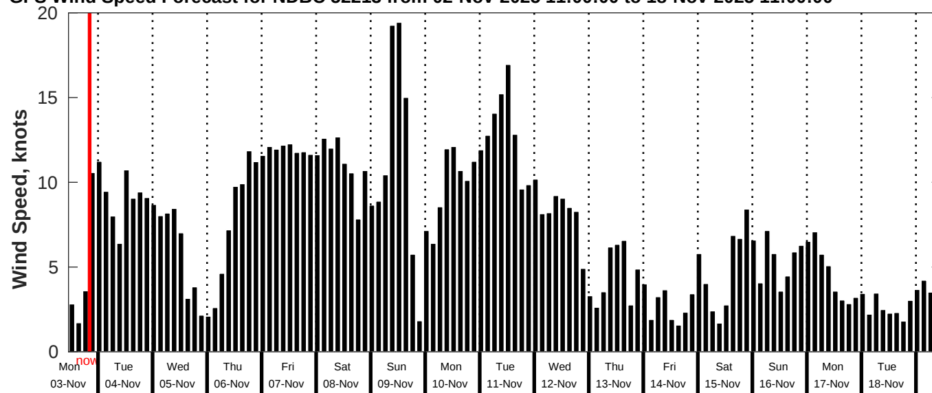
GFS Wind Speed Forecast for NDBC 52213 from 02-Nov-2025 11:00:00 to 18-Nov-2025 11:00:00
