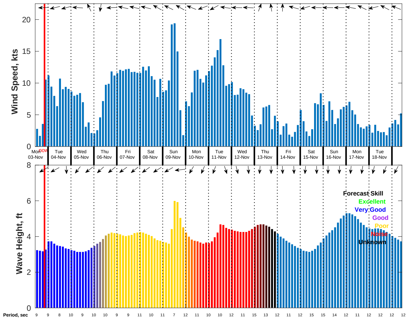
Wind & Wave Forecast for NDBC 52213 from 02-Nov-2025 11:00:00 to 18-Nov-2025 11:00:00
