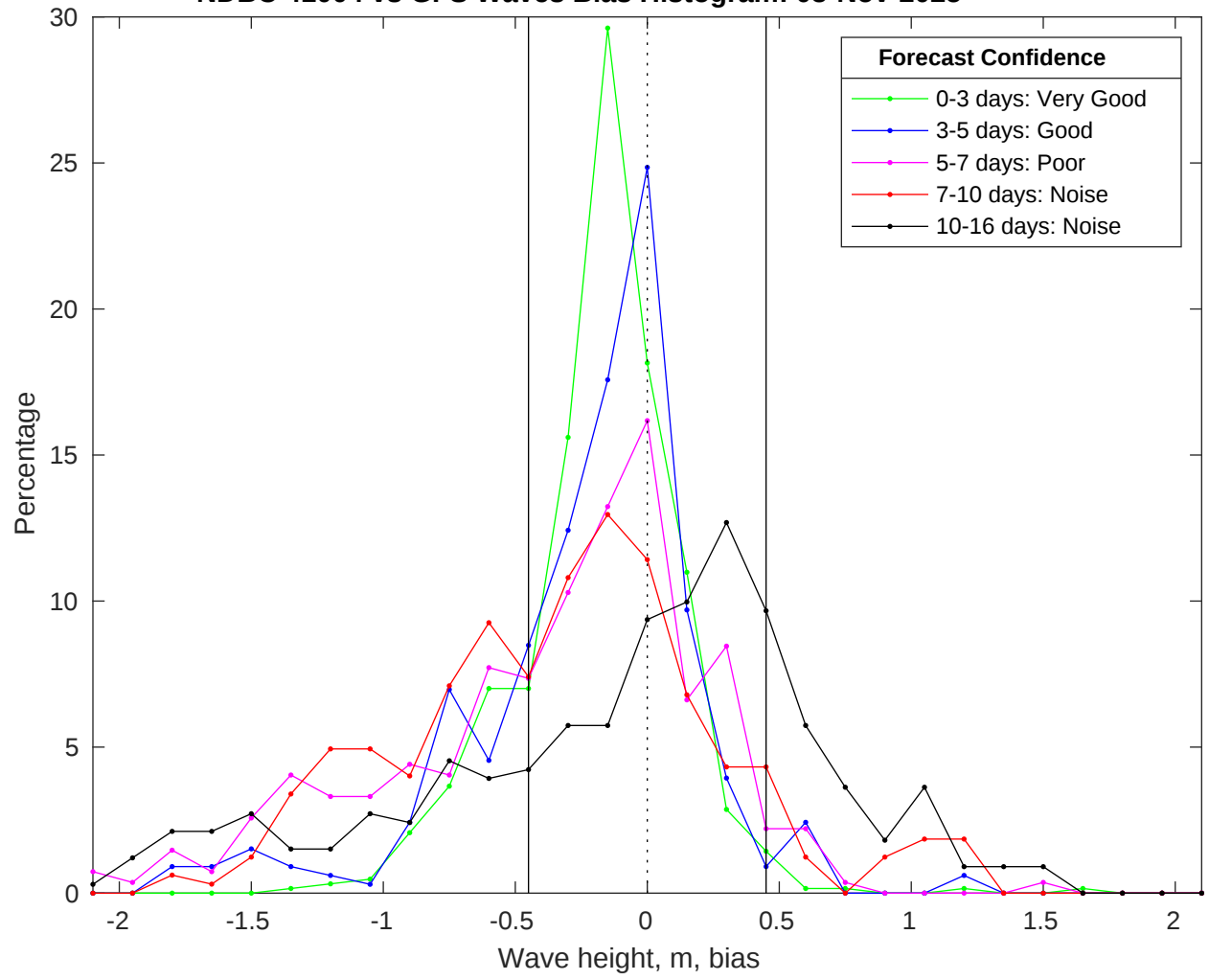
NDBC 41004 vs GFS Waves Bias Histogram: 03-Nov-2025
