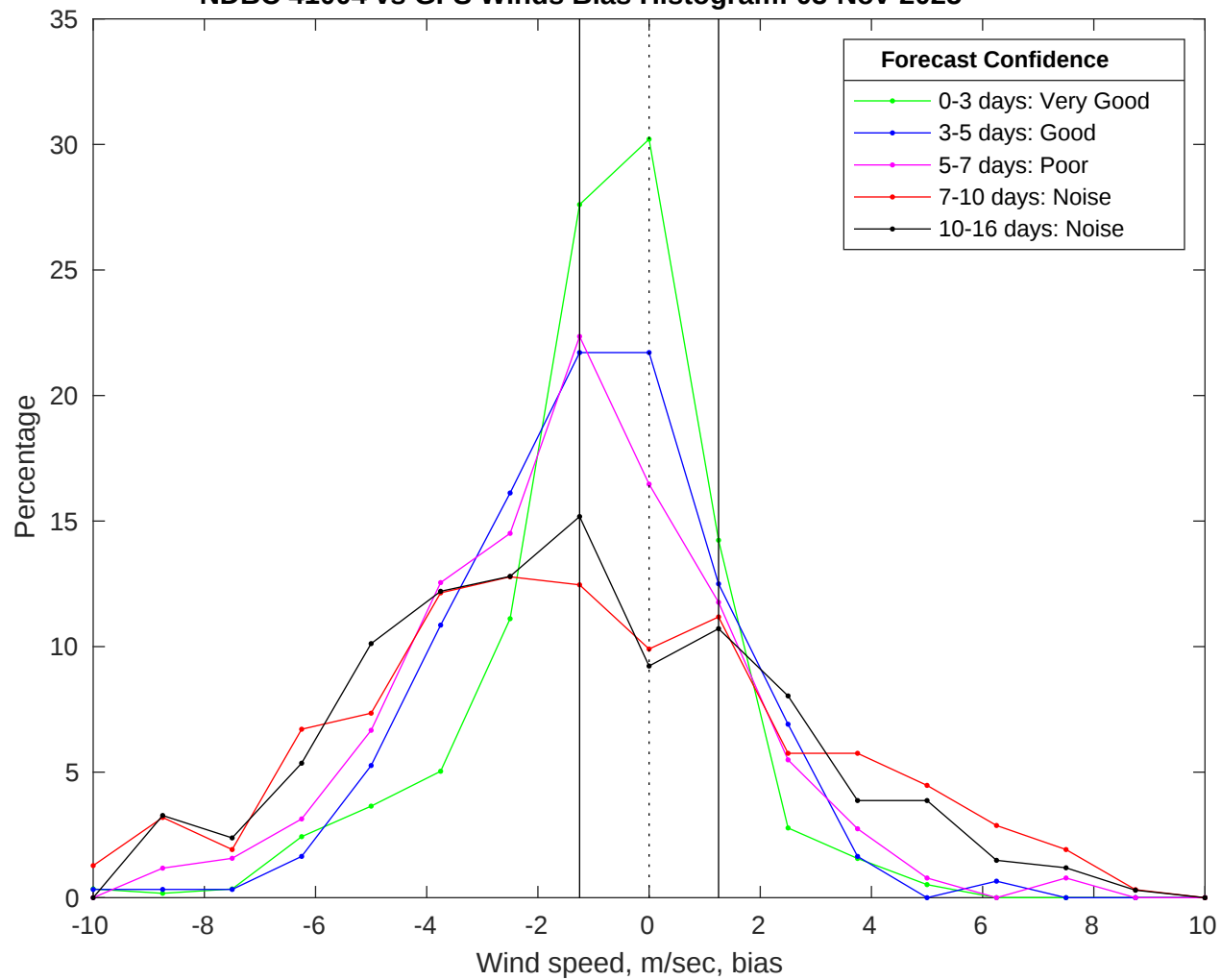
NDBC 41004 vs GFS Winds Bias Histogram: 03-Nov-2025
