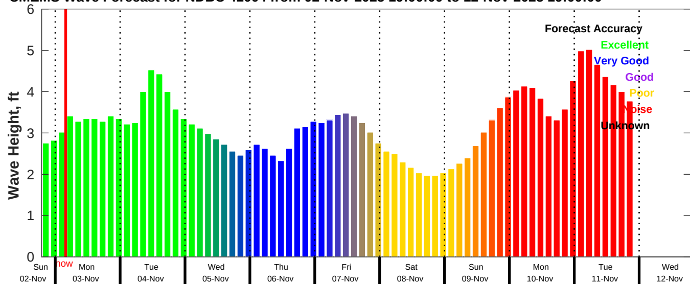
CMEMS Wave Forecast for NDBC 41004 from 02-Nov-2025 19:00:00 to 12-Nov-2025 19:00:00
