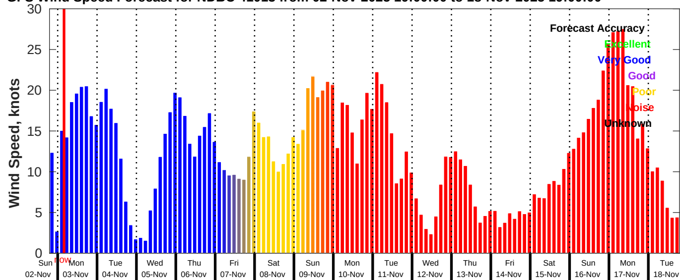
GFS Wind Speed Forecast for NDBC 41013 from 02-Nov-2025 19:00:00 to 18-Nov-2025 19:00:00
