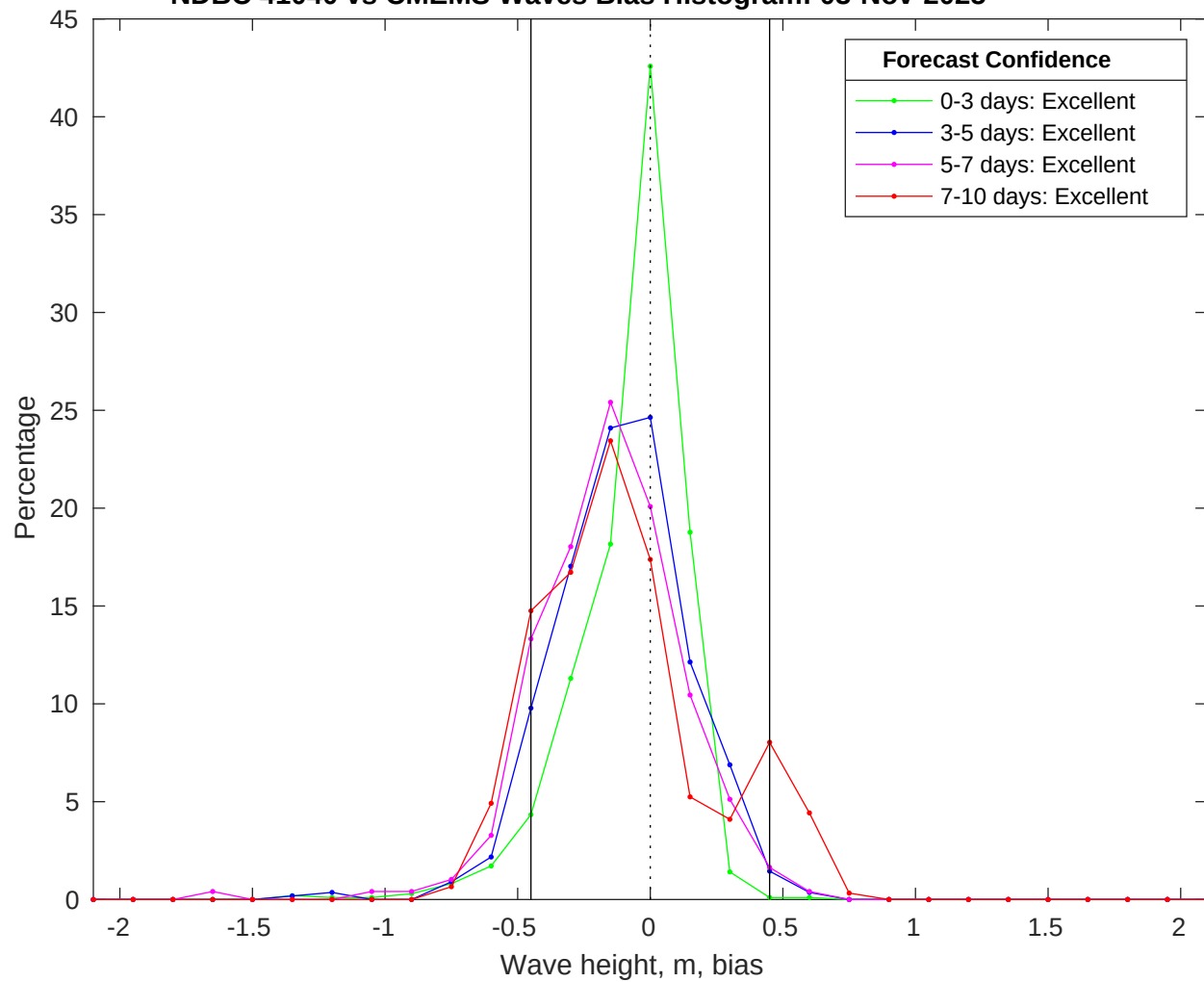
NDBC 41040 vs CMEMS Waves Bias Histogram: 03-Nov-2025
