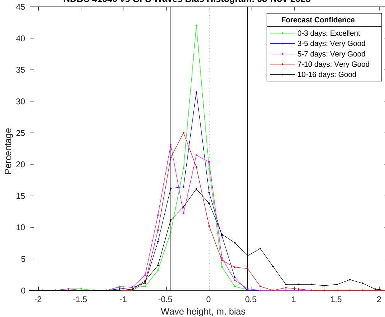
NDBC 41040 vs GFS Waves Bias Histogram: 03-Nov-2025
