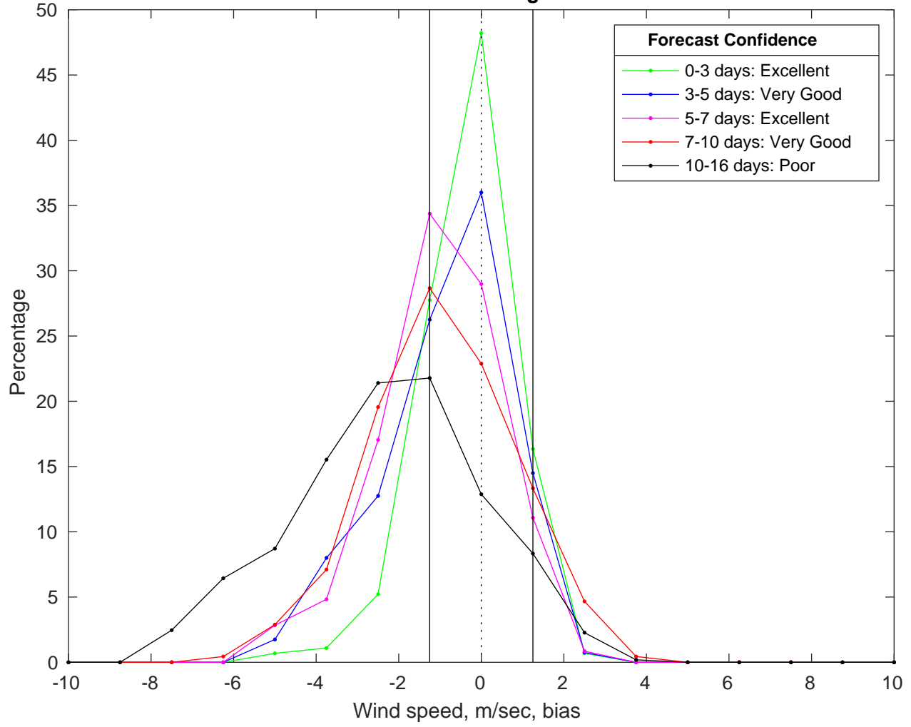
NDBC 41040 vs GFS Winds Bias Histogram: 03-Nov-2025
