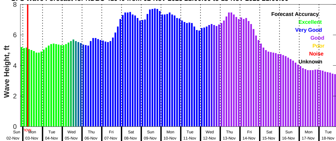
GFS Wave Forecast for NDBC 41040 from 02-Nov-2025 21:00:00 to 18-Nov-2025 21:00:00
