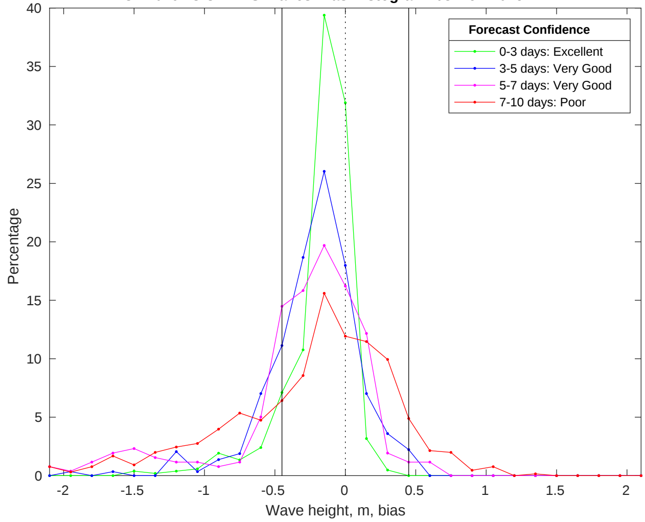
NDBC 42019 vs CMEMS Waves Bias Histogram: 03-Nov-2025
