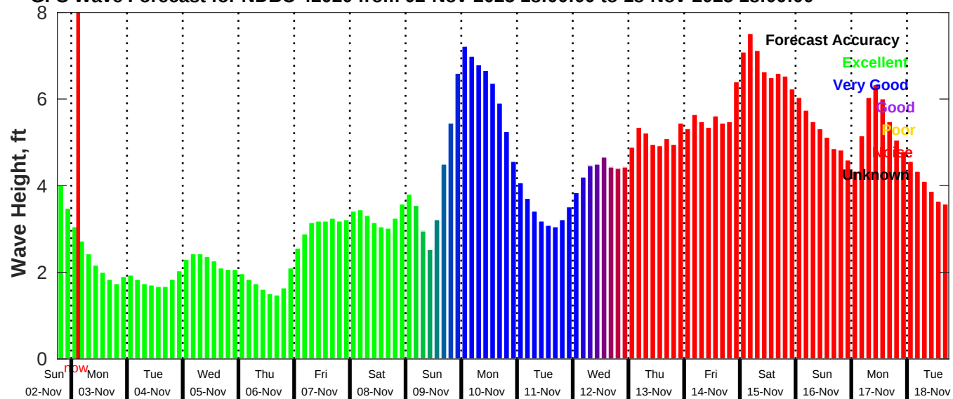
GFS Wave Forecast for NDBC 42020 from 02-Nov-2025 18:00:00 to 18-Nov-2025 18:00:00
