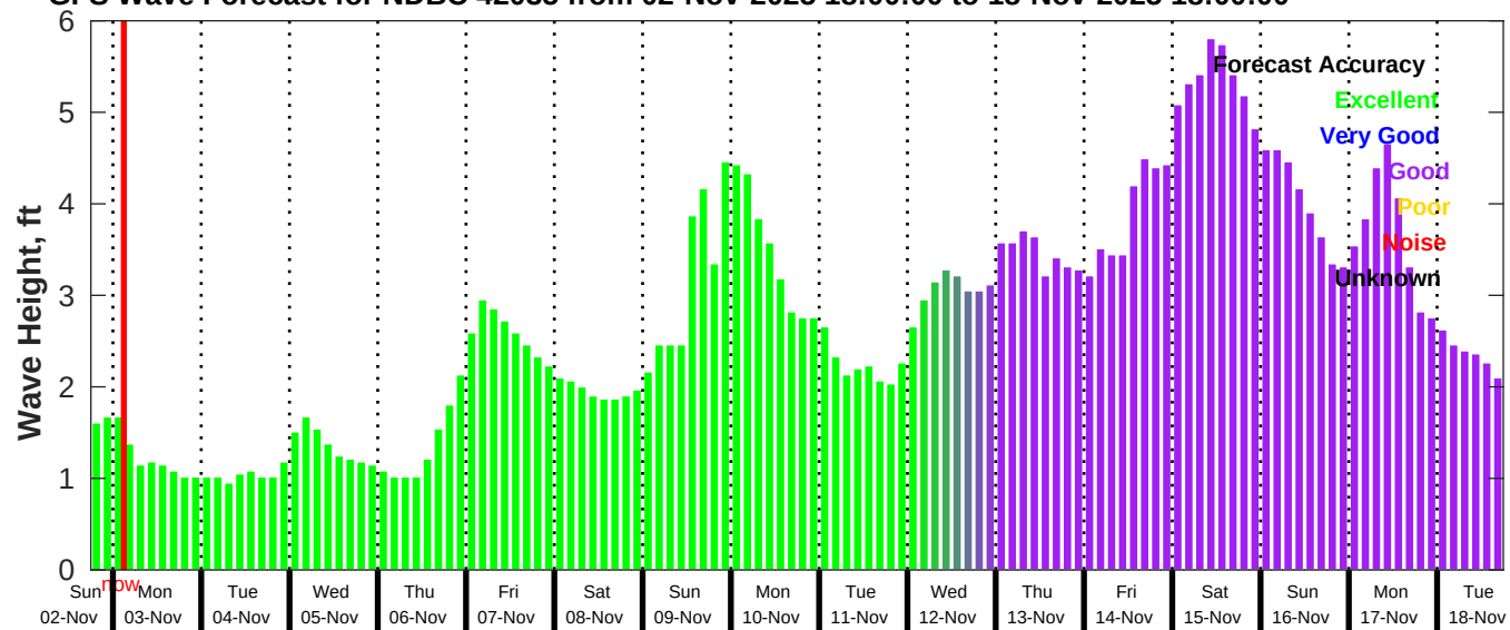
GFS Wave Forecast for NDBC 42035 from 02-Nov-2025 18:00:00 to 18-Nov-2025 18:00:00
