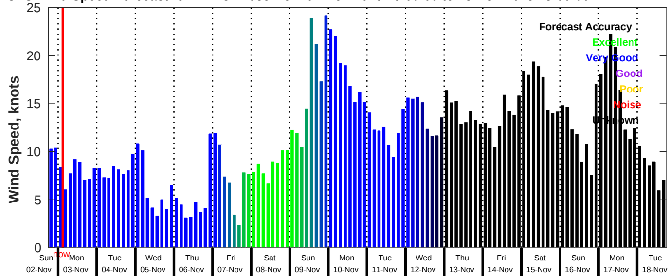
GFS Wind Speed Forecast for NDBC 42035 from 02-Nov-2025 18:00:00 to 18-Nov-2025 18:00:00
