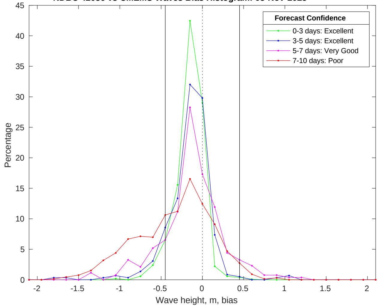
NDBC 42036 vs CMEMS Waves Bias Histogram: 03-Nov-2025
