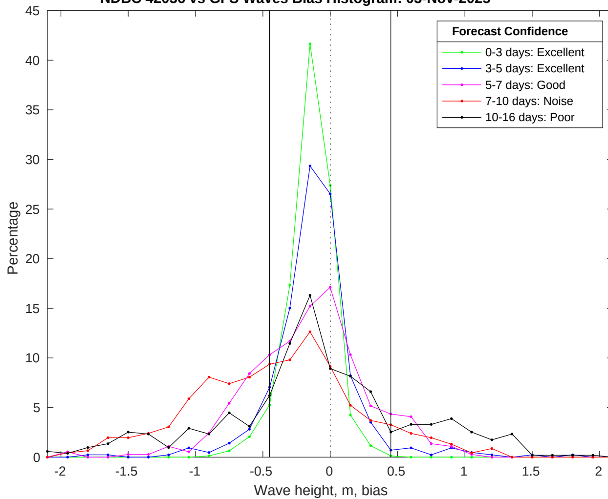
NDBC 42036 vs GFS Waves Bias Histogram: 03-Nov-2025
