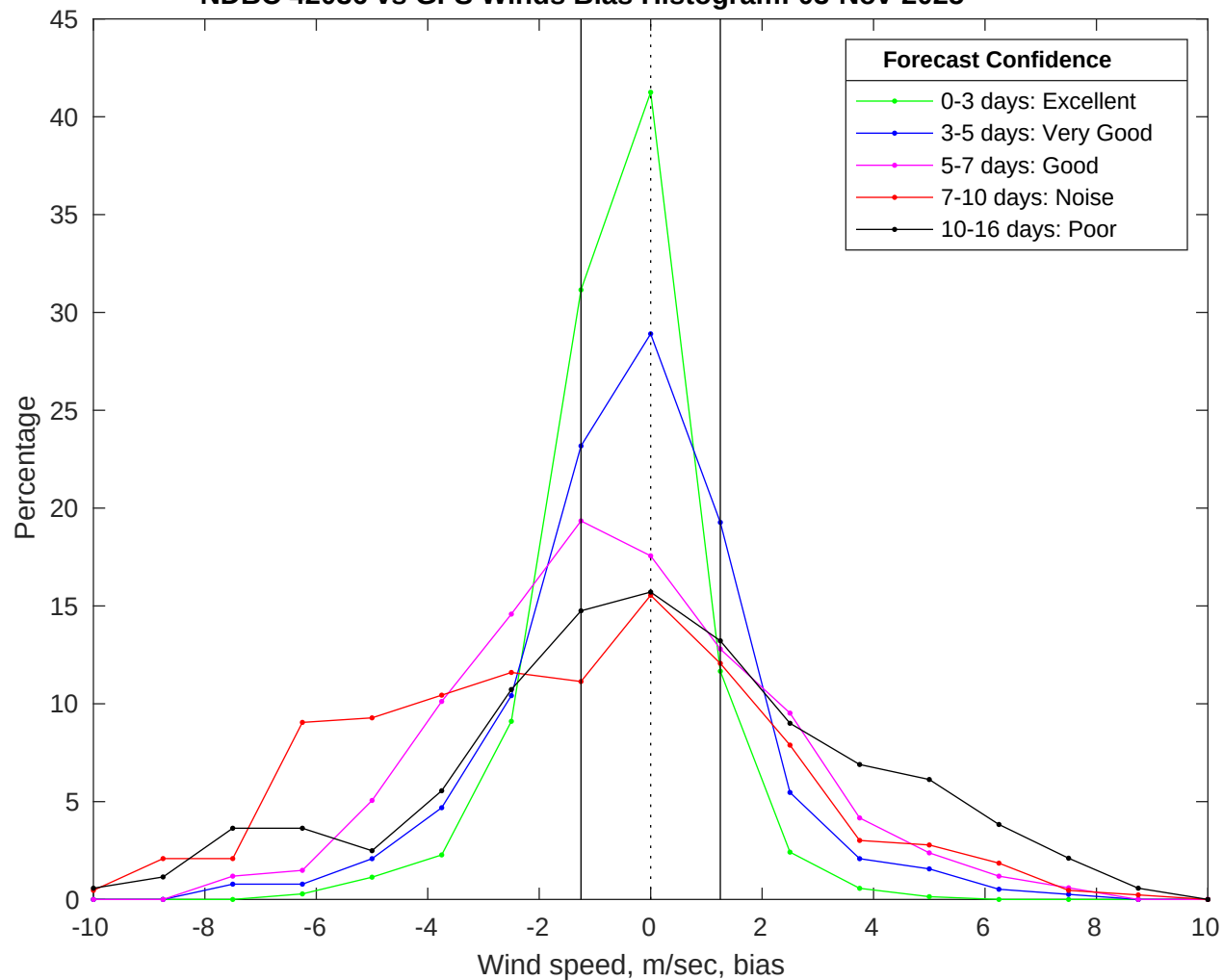
NDBC 42036 vs GFS Winds Bias Histogram: 03-Nov-2025
