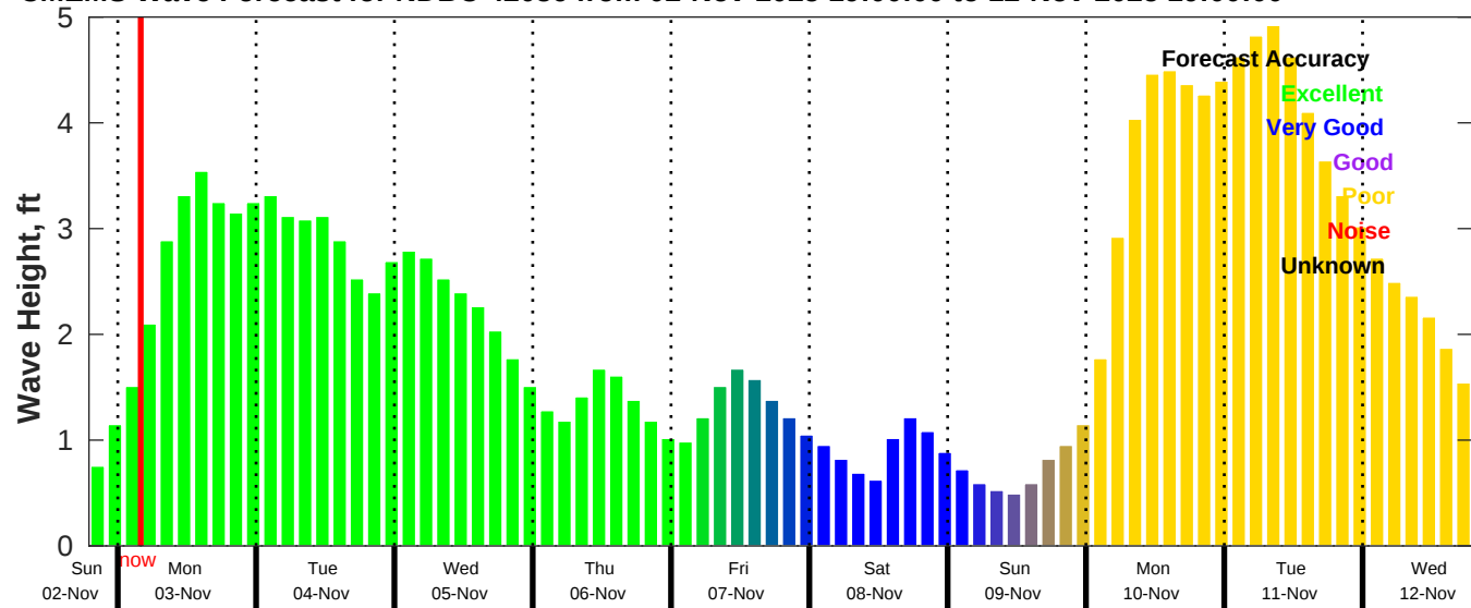
CMEMS Wave Forecast for NDBC 42036 from 02-Nov-2025 19:00:00 to 12-Nov-2025 19:00:00
