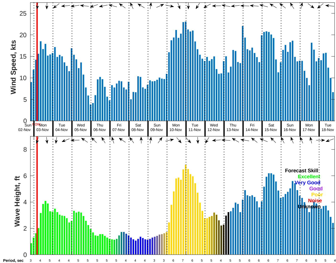
Wind & Wave Forecast for NDBC 42036 from 02-Nov-2025 19:00:00 to 18-Nov-2025 19:00:00
