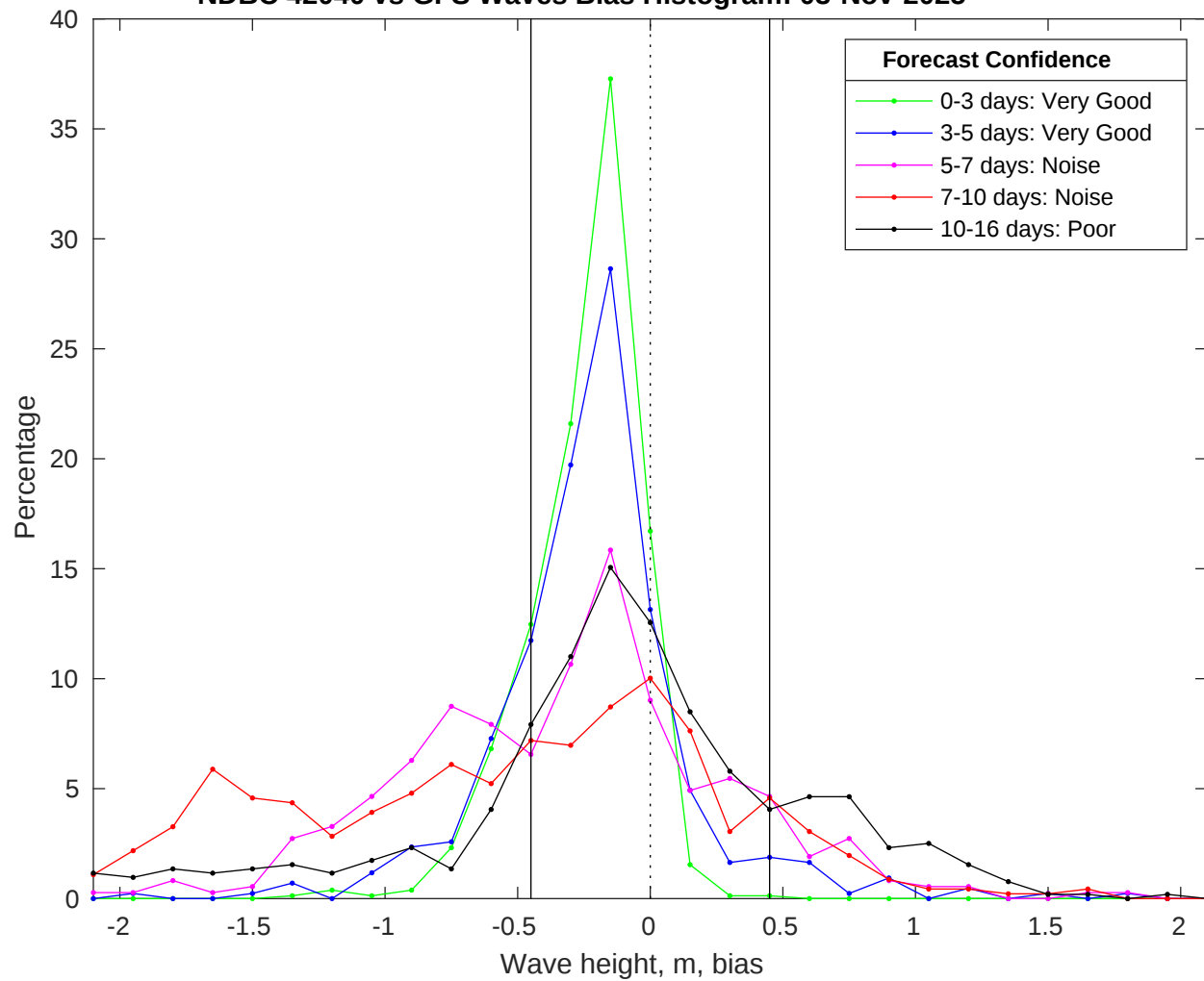
NDBC 42040 vs GFS Waves Bias Histogram: 03-Nov-2025
