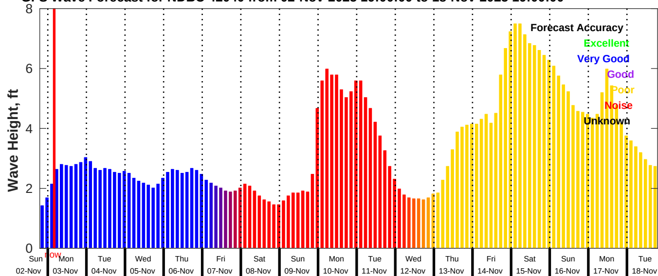
GFS Wave Forecast for NDBC 42040 from 02-Nov-2025 19:00:00 to 18-Nov-2025 19:00:00
