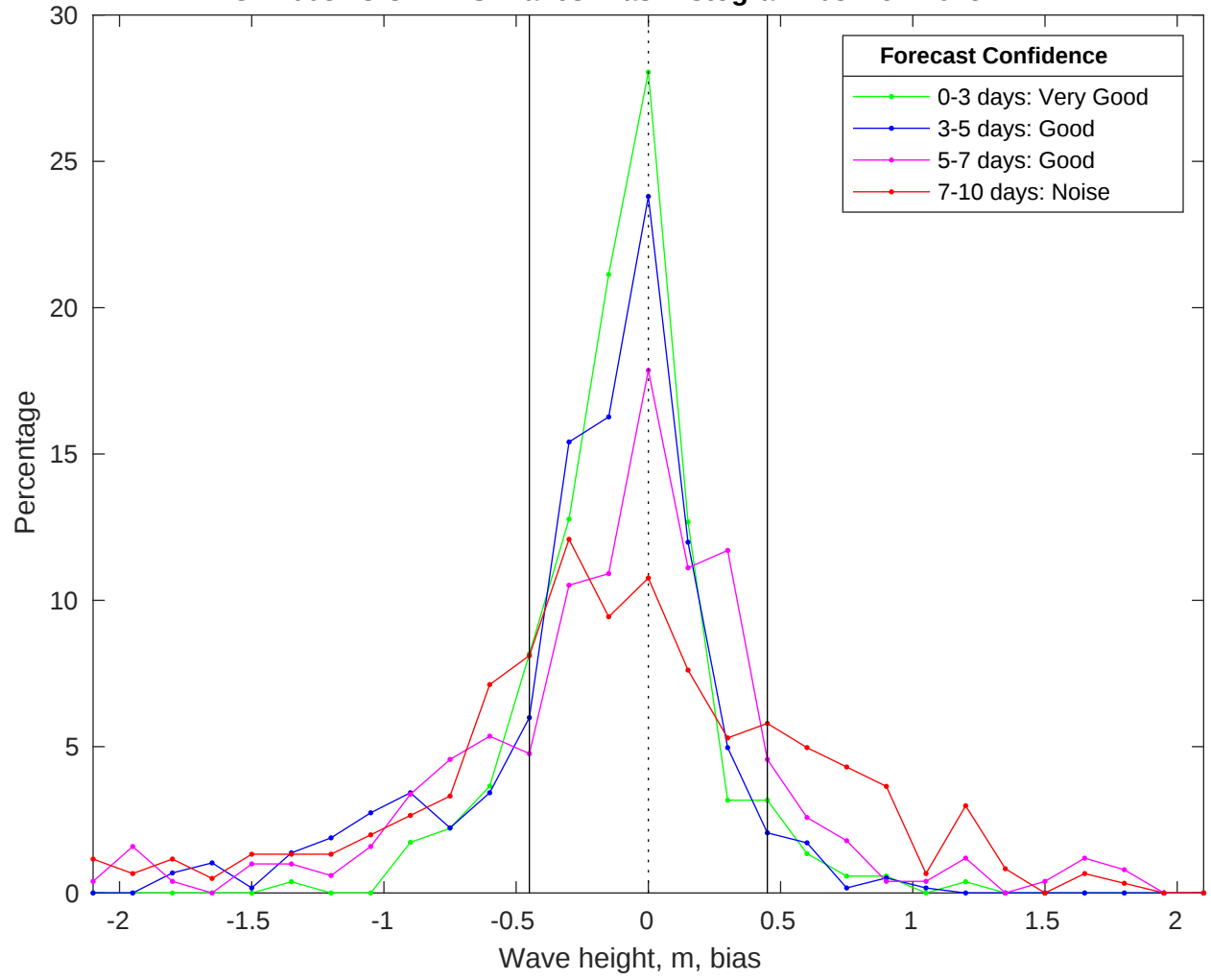
NDBC 44008 vs CMEMS Waves Bias Histogram: 03-Nov-2025
