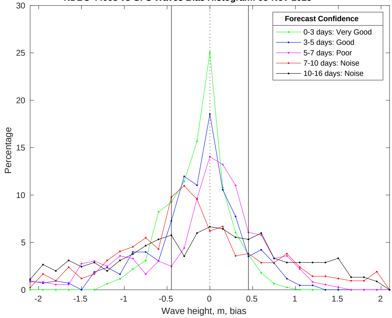
NDBC 44008 vs GFS Waves Bias Histogram: 03-Nov-2025
