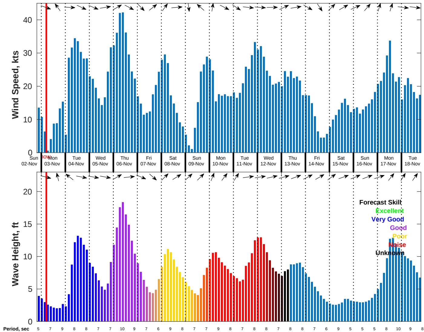
Wind & Wave Forecast for NDBC 44008 from 02-Nov-2025 20:00:00 to 18-Nov-2025 20:00:00
