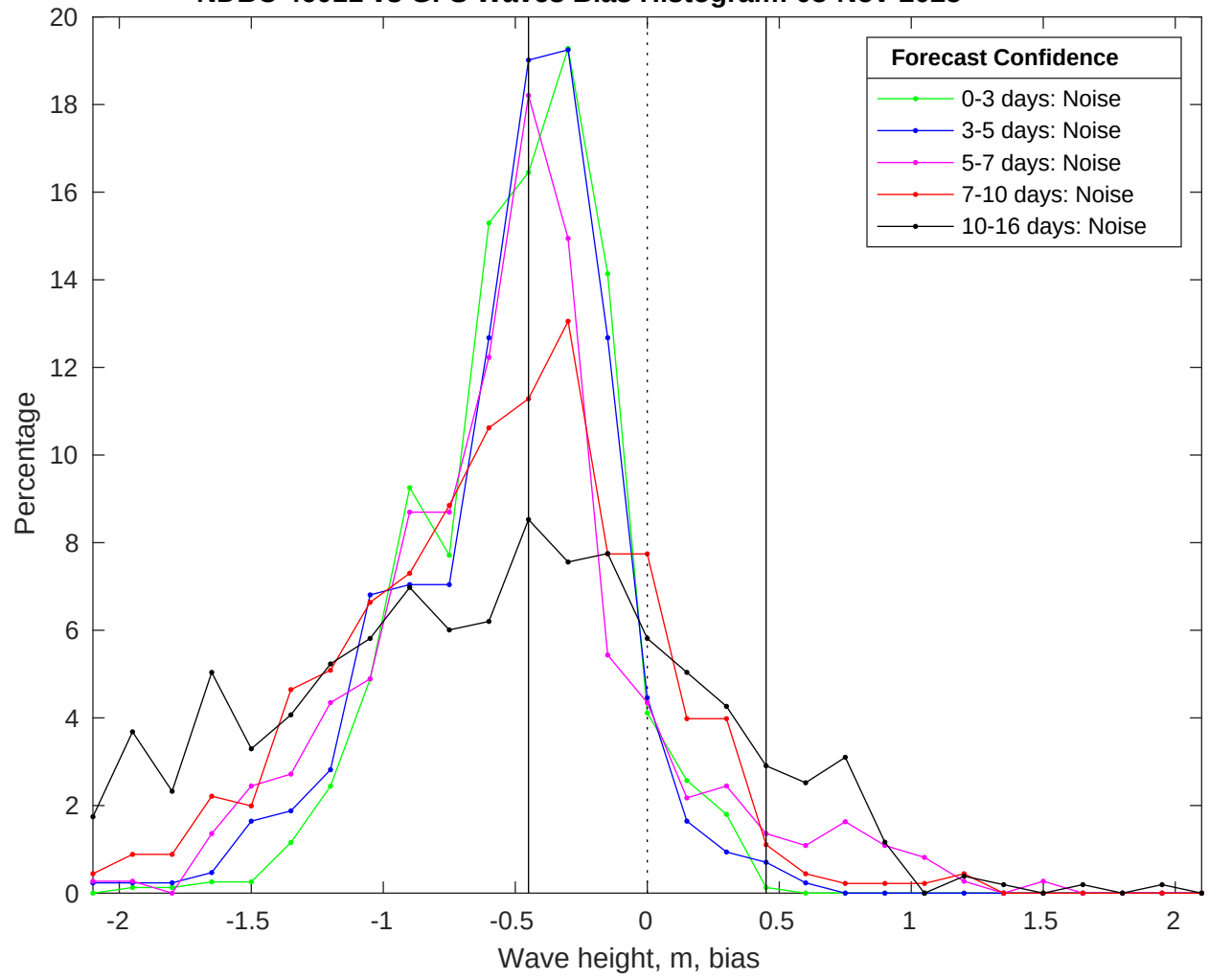
NDBC 46011 vs GFS Waves Bias Histogram: 03-Nov-2025
