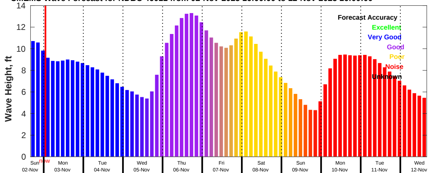
CMEMS Wave Forecast for NDBC 46011 from 02-Nov-2025 16:00:00 to 12-Nov-2025 16:00:00
