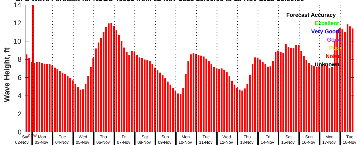
GFS Wave Forecast for NDBC 46011 from 02-Nov-2025 16:00:00 to 18-Nov-2025 16:00:00
