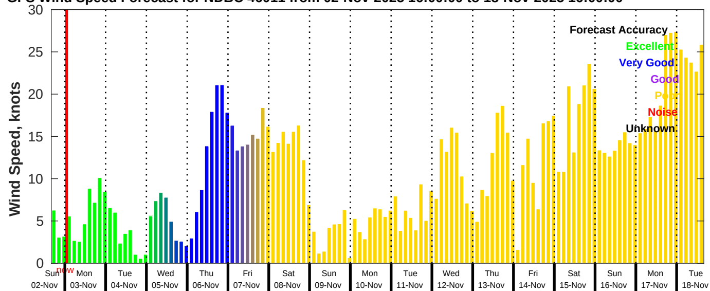
GFS Wind Speed Forecast for NDBC 46011 from 02-Nov-2025 16:00:00 to 18-Nov-2025 16:00:00
