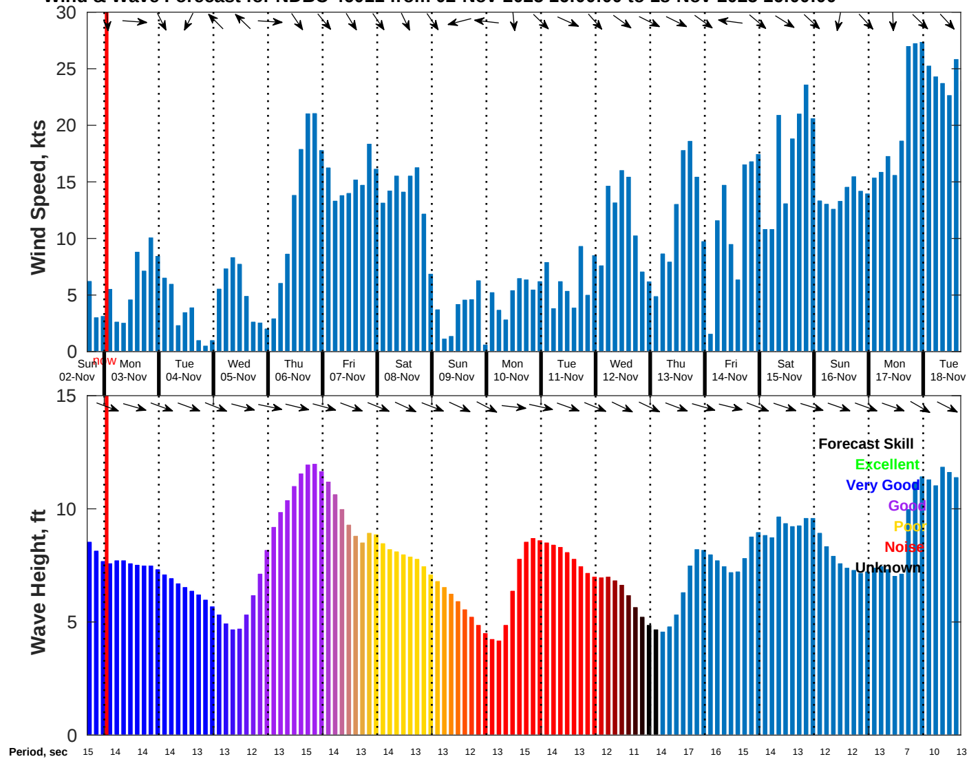
Wind & Wave Forecast for NDBC 46011 from 02-Nov-2025 16:00:00 to 18-Nov-2025 16:00:00
