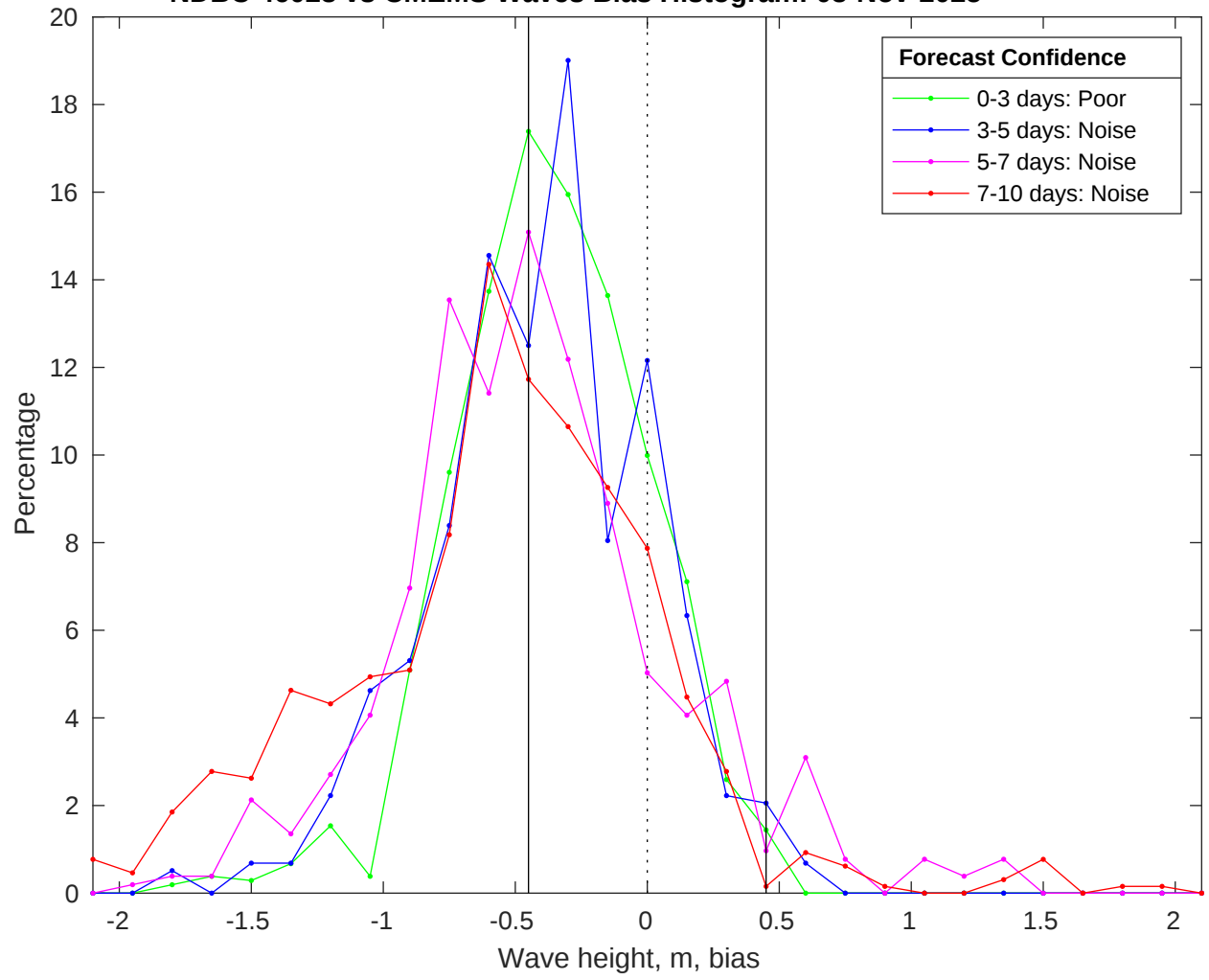
NDBC 46028 vs CMEMS Waves Bias Histogram: 03-Nov-2025
