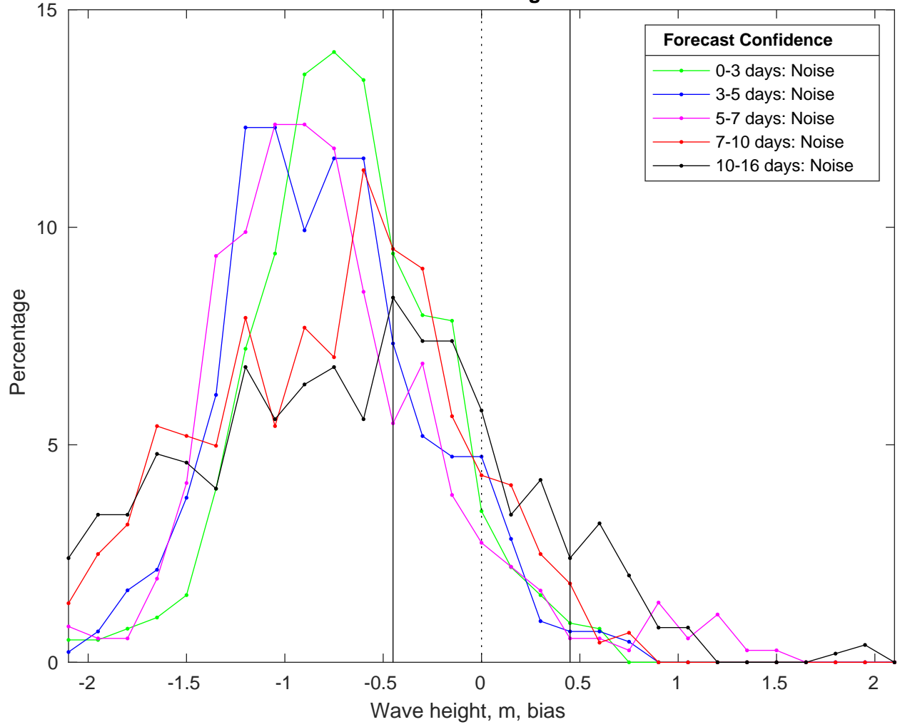
NDBC 46028 vs GFS Waves Bias Histogram: 03-Nov-2025
